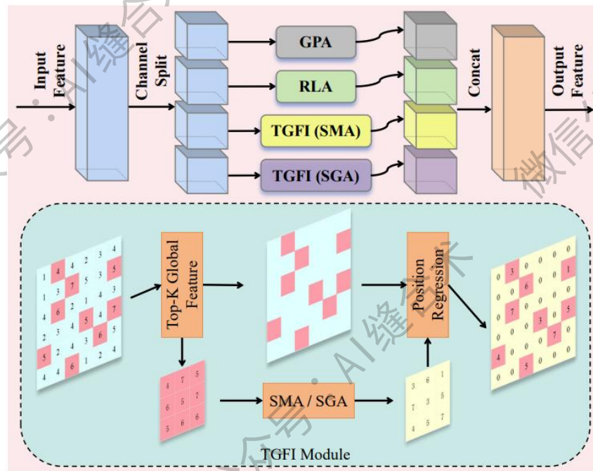
Fig. 3: Illustration of LWGA module.
